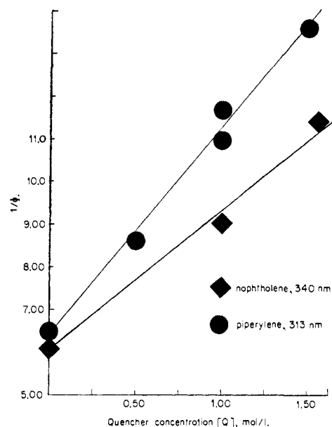
Figure 2. Stern-Volmer plot; appearance of cis -3- p -methoxyphenyl- trans -2-phenyl-1-benzoylcyclopropane.
