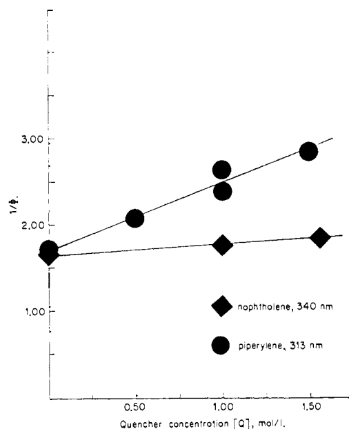
Figure 3. Stern-Volmer plot; appearance of trans -3- p -methoxyphenyl- cis -2-phenyl-1-benzoylcyclopropane.
