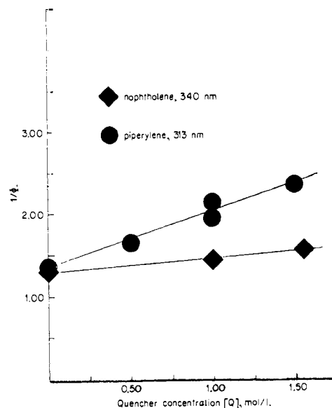
Figure 1. Stern-Volmer plot; disappearance of trans -3- p -methoxyphenyl- trans -2-phenyl-1-benzoylcyclopropane.
